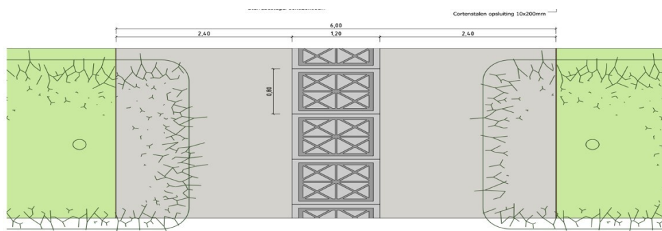
Detail Sterrebospad As Martinitorren Schaal 1:50
