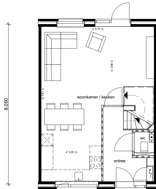
6.000 type A basis Begane grond kavel 1 t/m 8
