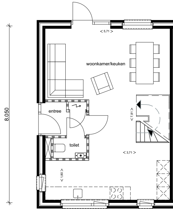
6.000 type F basis Begane grond kavel 9
